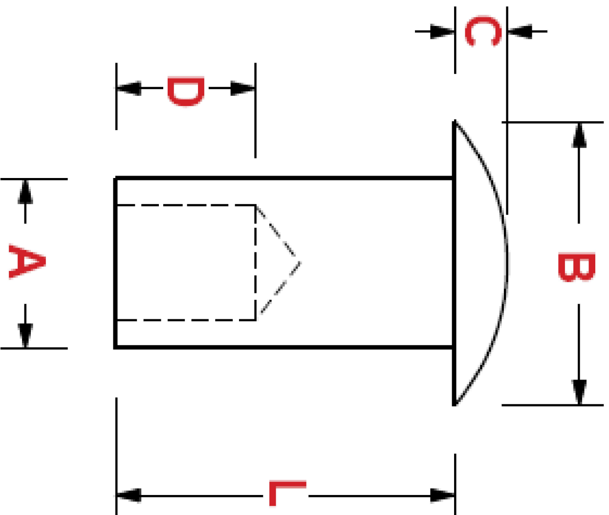
SEMI-TUBULAR RIVETS STANDARD OVAL HEAD
